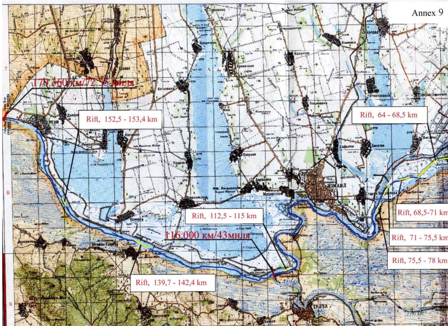
Scheme of Deep Water Navigation Route
